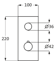
LARIMAR UP-Thermostat, 1 Blende eckig, 1 Absperrventil, 2 Griffe rund, chrom, LA433210500
