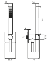
LARIMAR E1 Wannen-Brause Set intrg. Brauseh., Stabhandbr., chrom LA453160500
