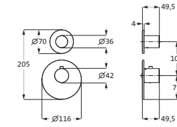
UP-Thermostat, 2 Blenden rund, 1 Absperrventil, 2 Griffe rund, chrom, LA433220500
