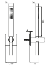
LARIMAR E1 Wannen-Brause Set Stabhandbrause, Schlauch 1250 mm, chrom LA453150500
