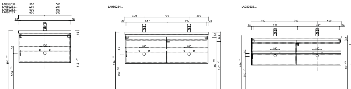
590 x 450 mm LA080230... 790 x 450 mm LA080231... 990 x 450 mm LA080232... 1290 x 450 mm LA080233... 1290 x 450 mm LA080234... 1490 x 450 mm LA080235...
